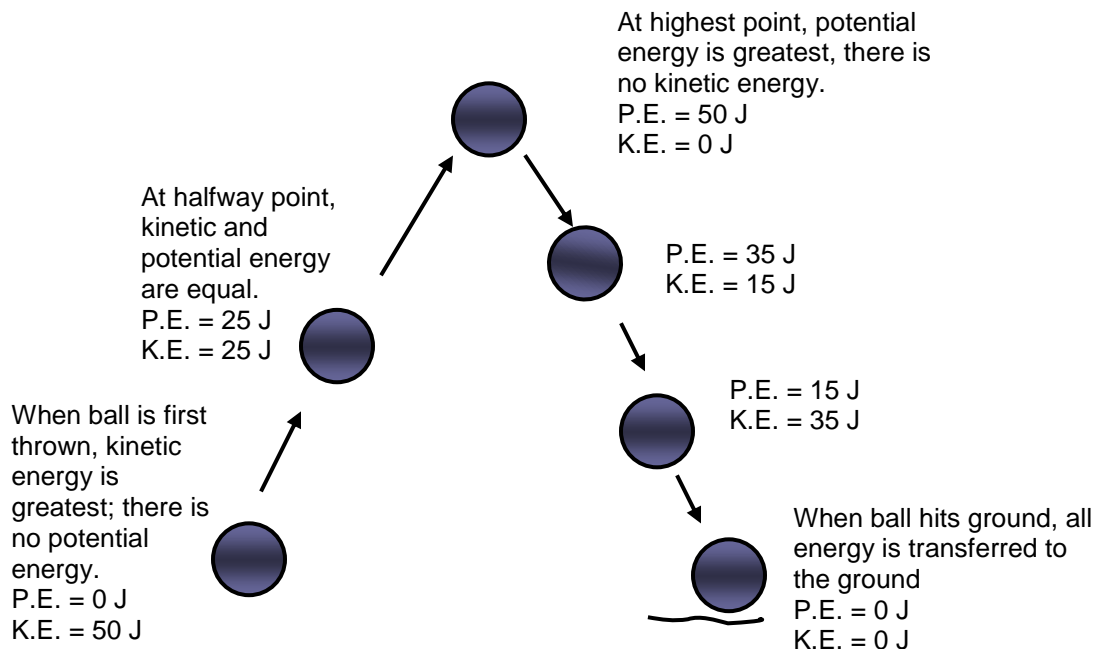
FIGURE 2: Kinetic and Potential Energy are Closely Related
