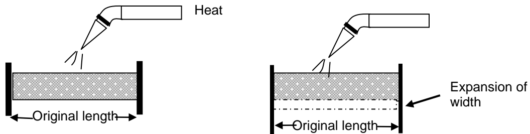
Figure 3A: Restricted metal cannot expand in length when heated
