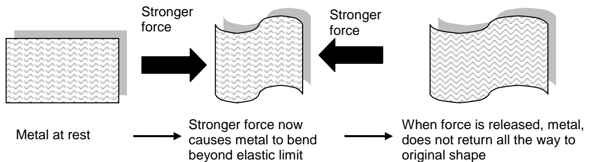
Figure 2: Plastic Deformation
