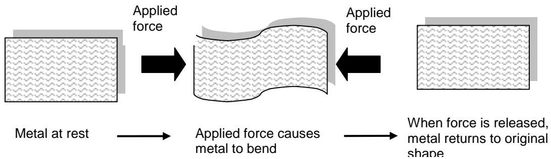
Figure 1: Elastic Deformation
