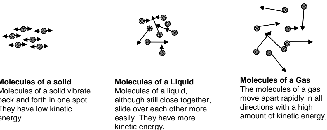
FIGURE 1: Molecular Motion and the Three Physical States Of Matter
